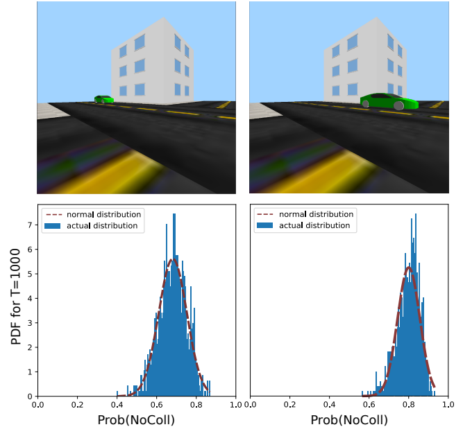
Fig. 1. Collision risk assessment via Deep Learning. Recent insights on Bayesian Deep Networks are used to generate a probability distribution. The histogram is computed out of 1000 stochastic forward passes.
